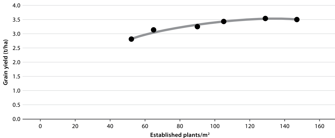
Figure 2. Grain yield response (t/ha) to number of plants established (plants/m 2 ) averaged over both seeders and row spacings in lentils. Density (P<0.01, LSD=0.2t/ha).
