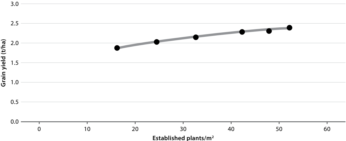
Figure 5. Grain yield response (t/ha) to number of plants established (plants/m 2 ) average over both seeders and row spacings in canola. Density: yield P<0.001, LSD 0.16t/ha.
